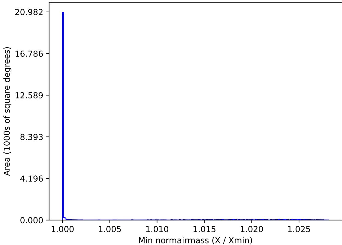
noroll_mjdp180_v3.4_10yrs All sky all bands: Min normairmass
