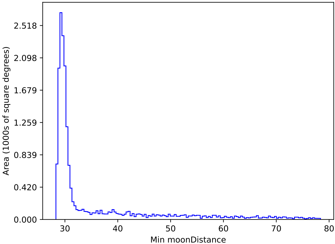
noroll_mjdp180_v3.4_10yrs WFD y band: Min moonDistance
