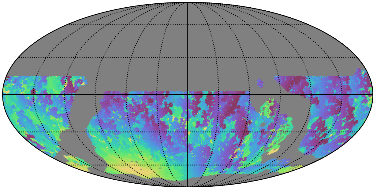
noroll_mjdp180_v3.4_10yrs WFD u band: Min moonDistance
