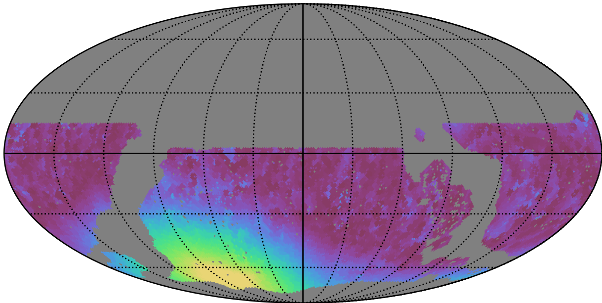
noroll_mjdp180_v3.4_10yrs WFD r band: Min moonDistance
