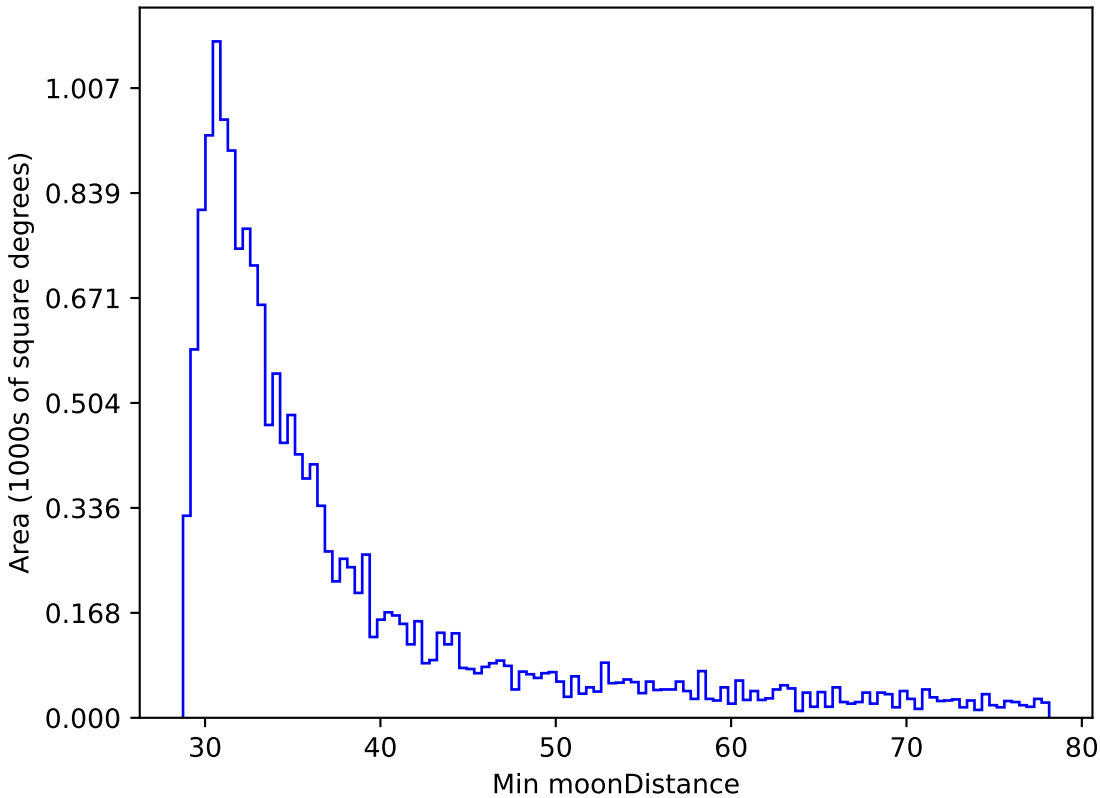
noroll_mjdp180_v3.4_10yrs WFD r band: Min moonDistance
