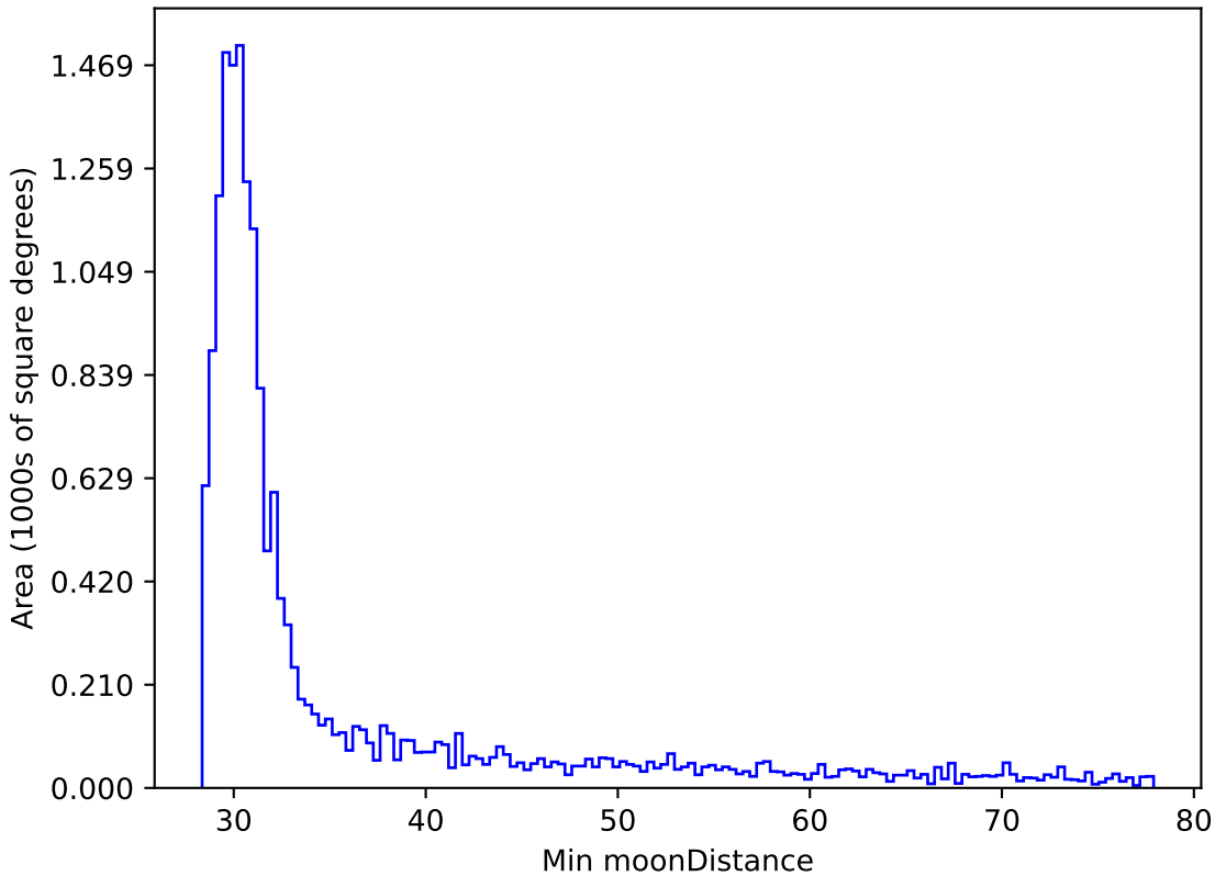
noroll_mjdp180_v3.4_10yrs WFD i band: Min moonDistance
