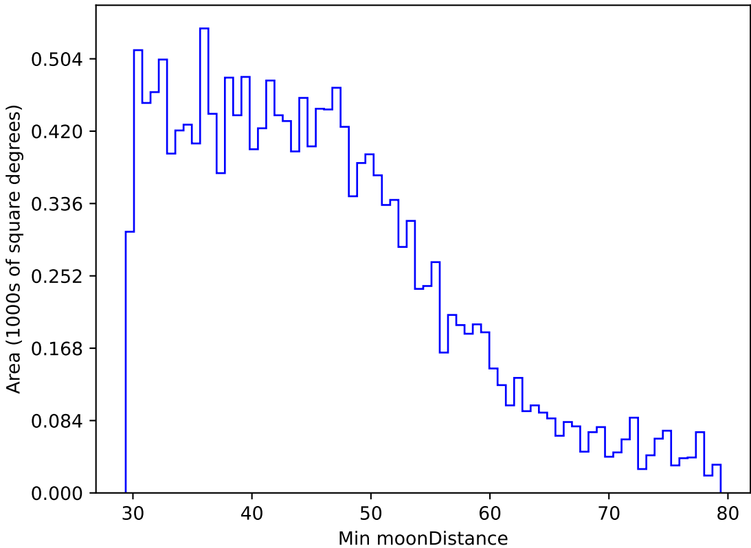
noroll_mjdp180_v3.4_10yrs WFD g band: Min moonDistance
