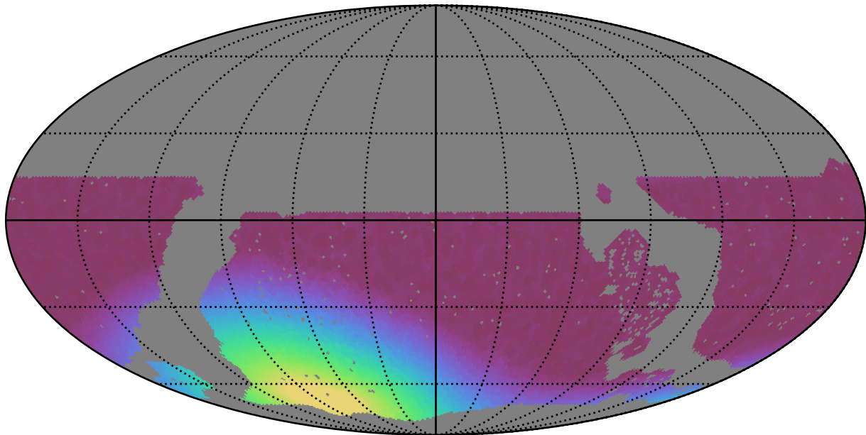
noroll_mjdp180_v3.4_10yrs WFD all bands: Min moonDistance
