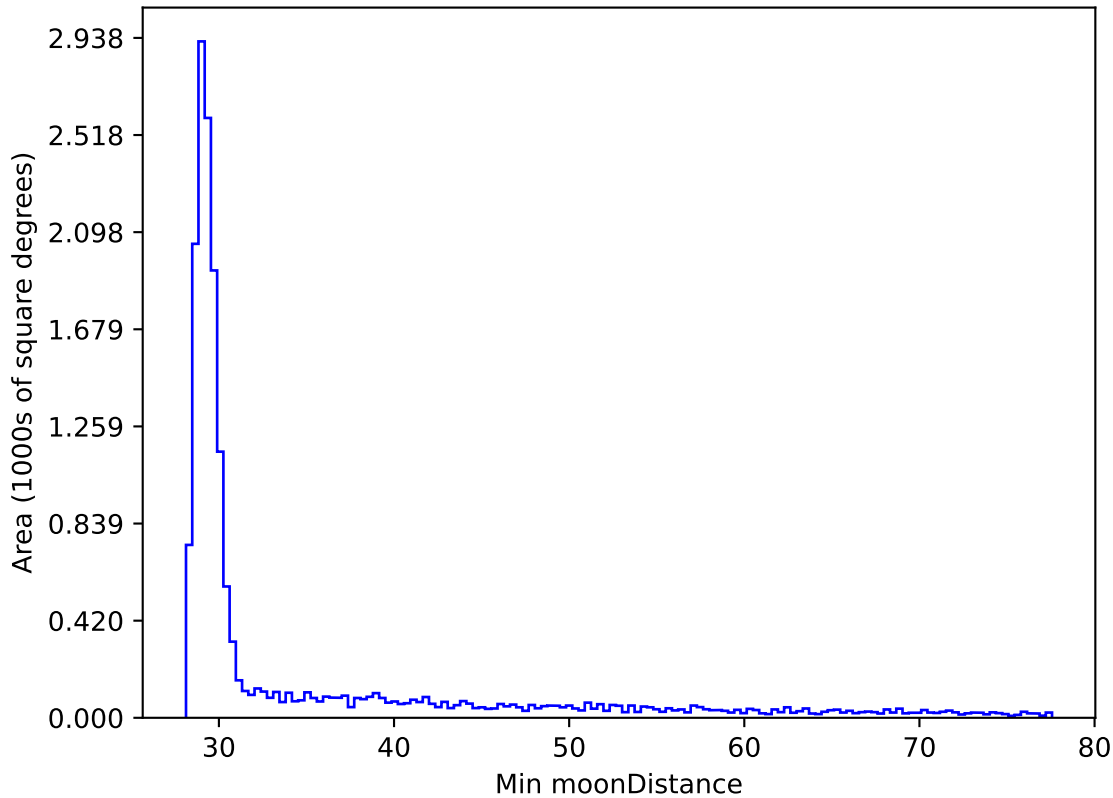
noroll_mjdp180_v3.4_10yrs WFD all bands: Min moonDistance
