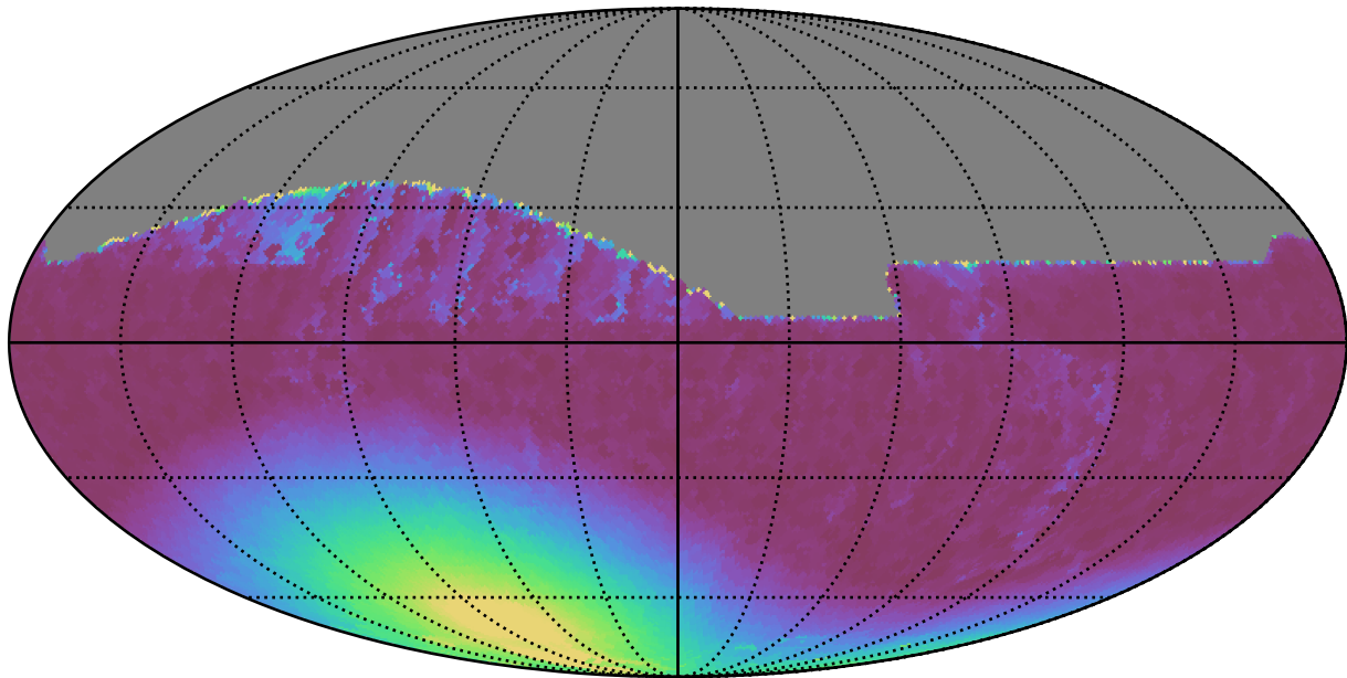
noroll_mjdp180_v3.4_10yrs All sky z band: Min moonDistance
