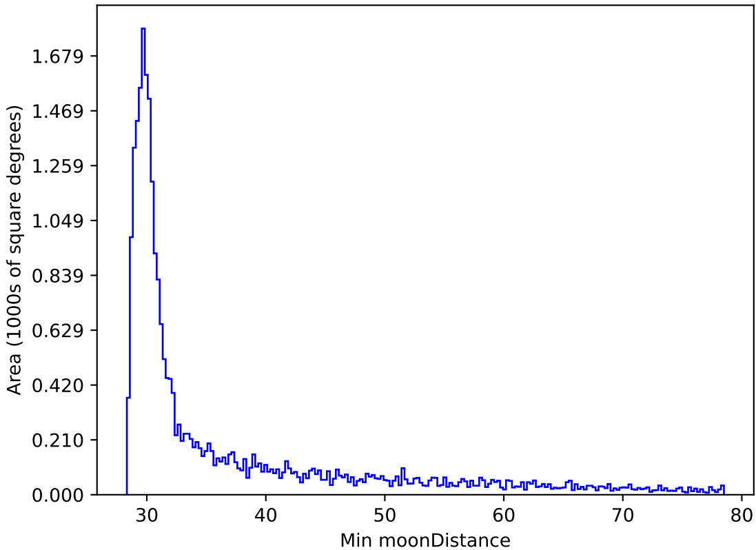
noroll_mjdp180_v3.4_10yrs All sky z band: Min moonDistance
