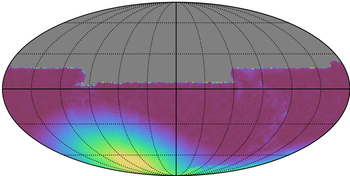
noroll_mjdp180_v3.4_10yrs All sky y band: Min moonDistance
