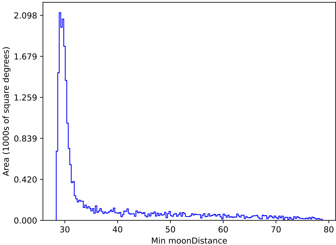
noroll_mjdp180_v3.4_10yrs All sky y band: Min moonDistance
