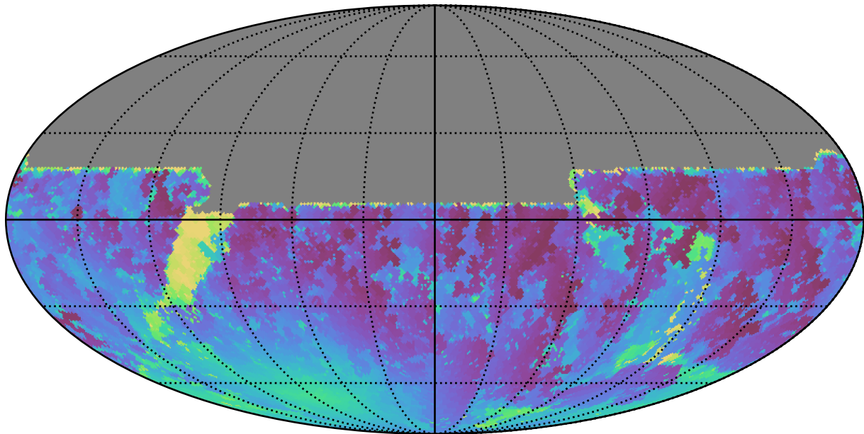
noroll_mjdp180_v3.4_10yrs All sky u band: Min moonDistance
