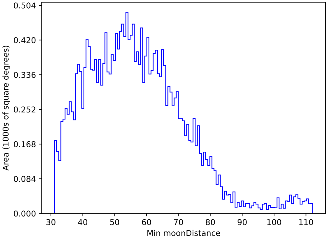
noroll_mjdp180_v3.4_10yrs All sky u band: Min moonDistance
