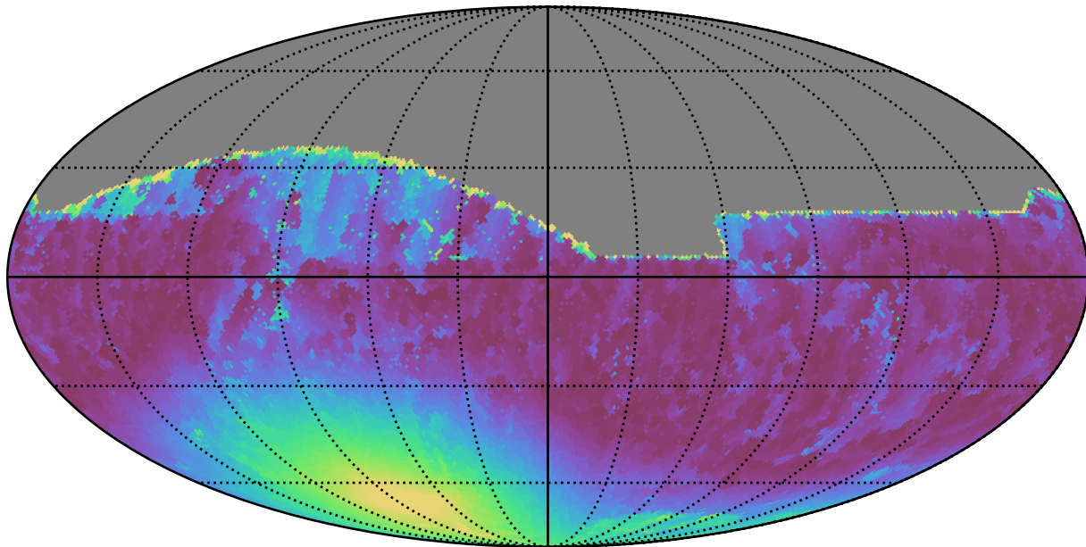
noroll_mjdp180_v3.4_10yrs All sky r band: Min moonDistance
