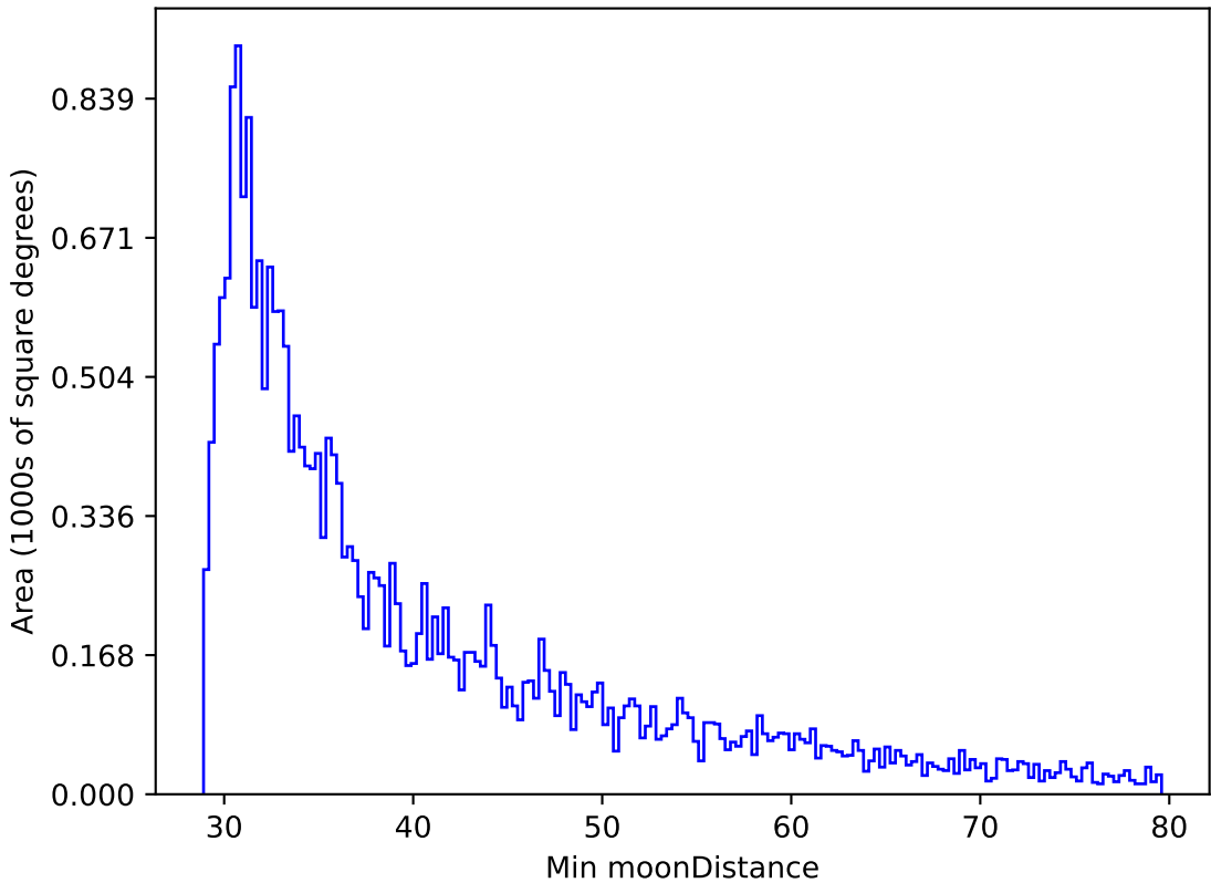
noroll_mjdp180_v3.4_10yrs All sky r band: Min moonDistance
