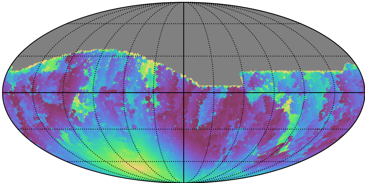
noroll_mjdp180_v3.4_10yrs All sky g band: Min moonDistance
