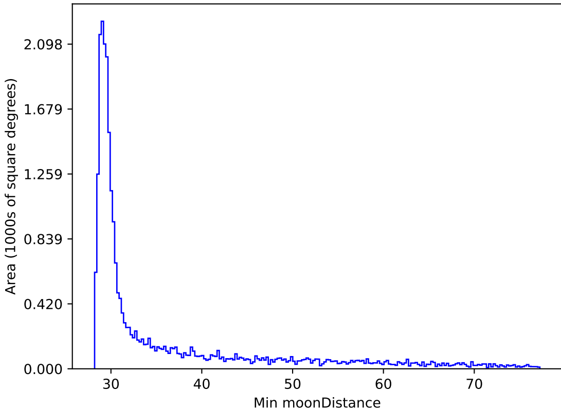
noroll_mjdp180_v3.4_10yrs All sky all bands: Min moonDistance
