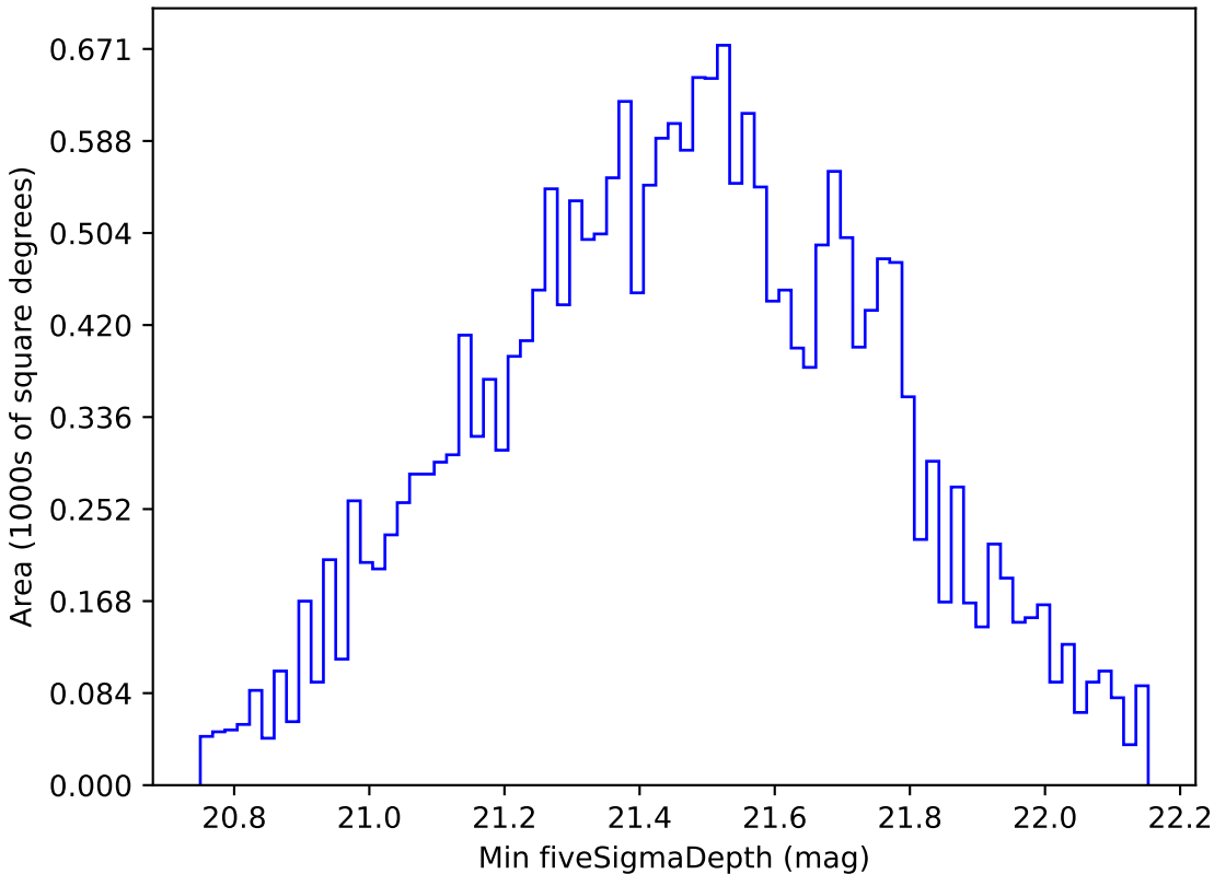
noroll_mjdp180_v3.4_10yrs Yr 1 y band: Min fiveSigmaDepth
