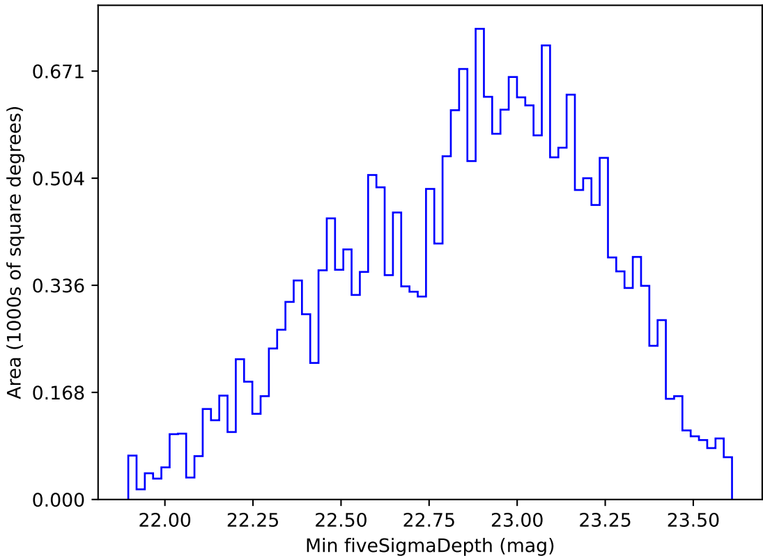
noroll_mjdp180_v3.4_10yrs Yr 1 u band: Min fiveSigmaDepth
