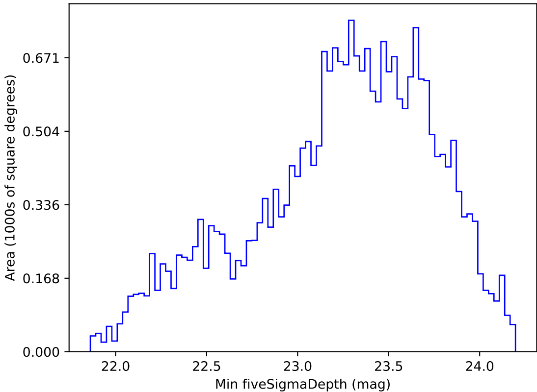
noroll_mjdp180_v3.4_10yrs Yr 1 r band: Min fiveSigmaDepth
