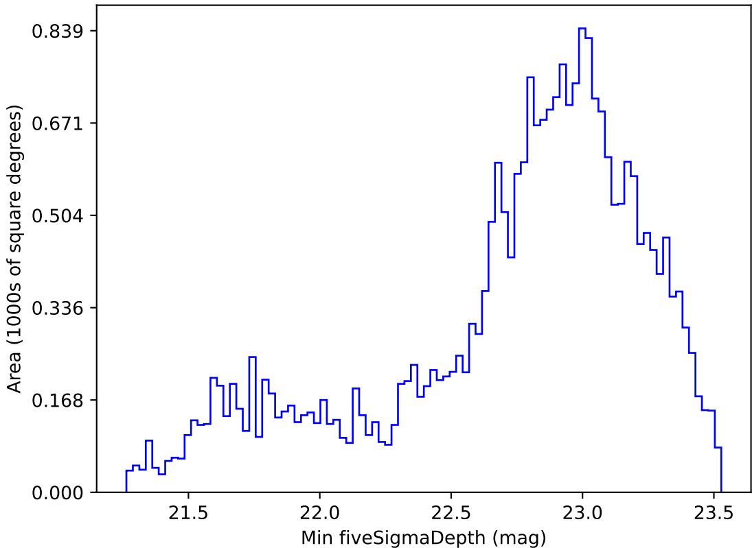
noroll_mjdp180_v3.4_10yrs Yr 1 i band: Min fiveSigmaDepth
