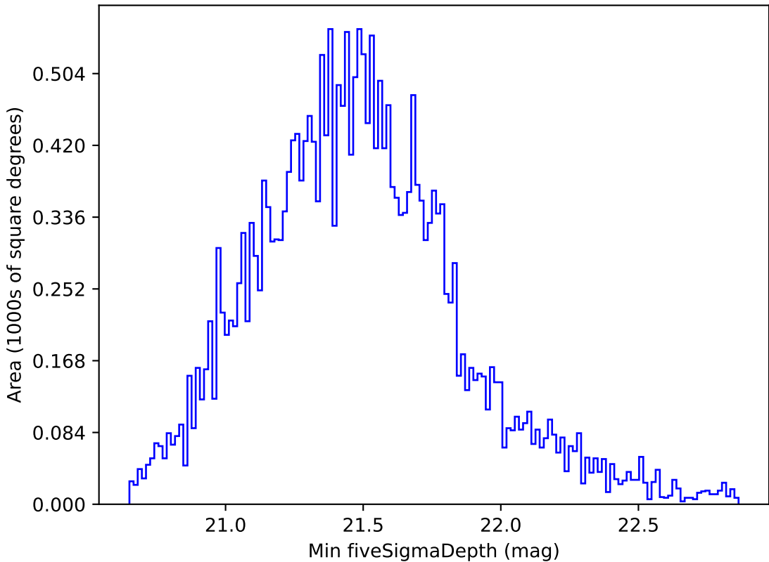
noroll_mjdp180_v3.4_10yrs Yr 1 all bands: Min fiveSigmaDepth
