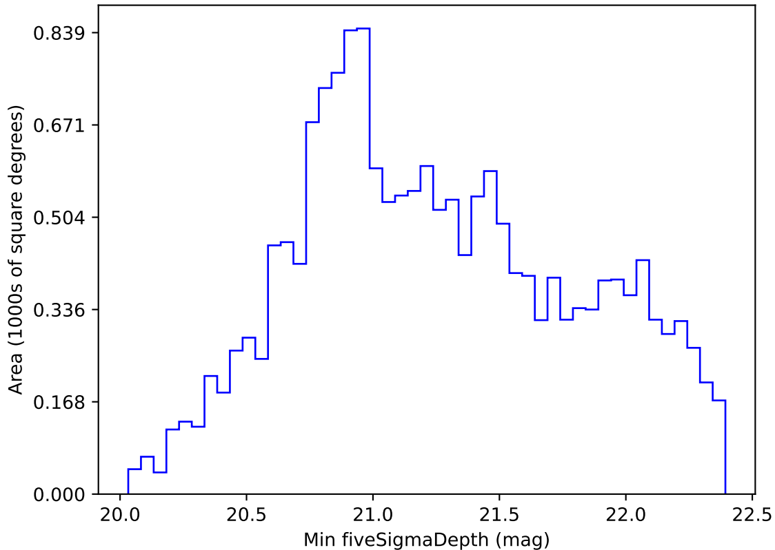
noroll_mjdp180_v3.4_10yrs WFD z band: Min fiveSigmaDepth
