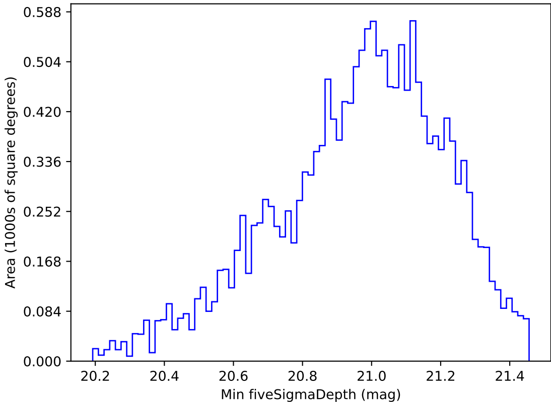
noroll_mjdp180_v3.4_10yrs WFD y band: Min fiveSigmaDepth
