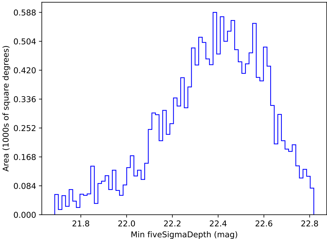
noroll_mjdp180_v3.4_10yrs WFD u band: Min fiveSigmaDepth
