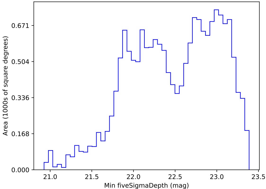
noroll_mjdp180_v3.4_10yrs WFD r band: Min fiveSigmaDepth
