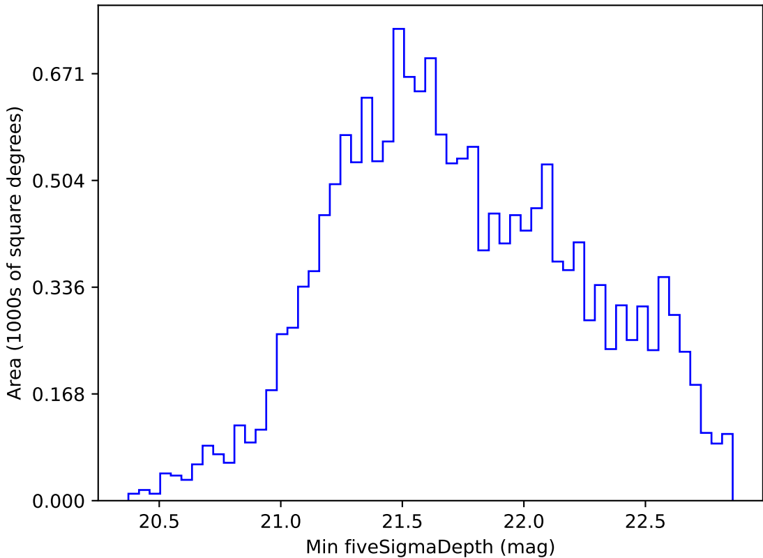
noroll_mjdp180_v3.4_10yrs WFD i band: Min fiveSigmaDepth
