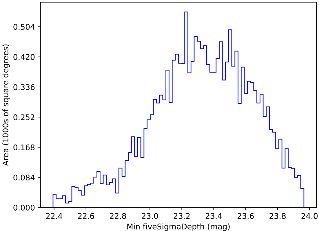
noroll_mjdp180_v3.4_10yrs WFD g band: Min fiveSigmaDepth
