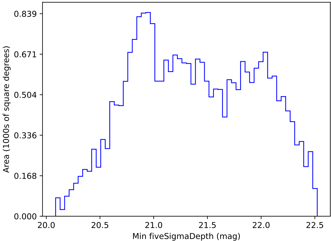
noroll_mjdp180_v3.4_10yrs All sky z band: Min fiveSigmaDepth
