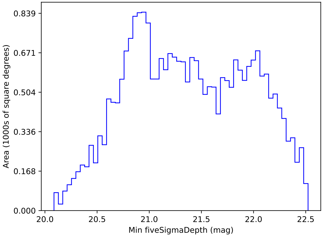
noroll_mjdp180_v3.4_10yrs All sky z band: Min fiveSigmaDepth
