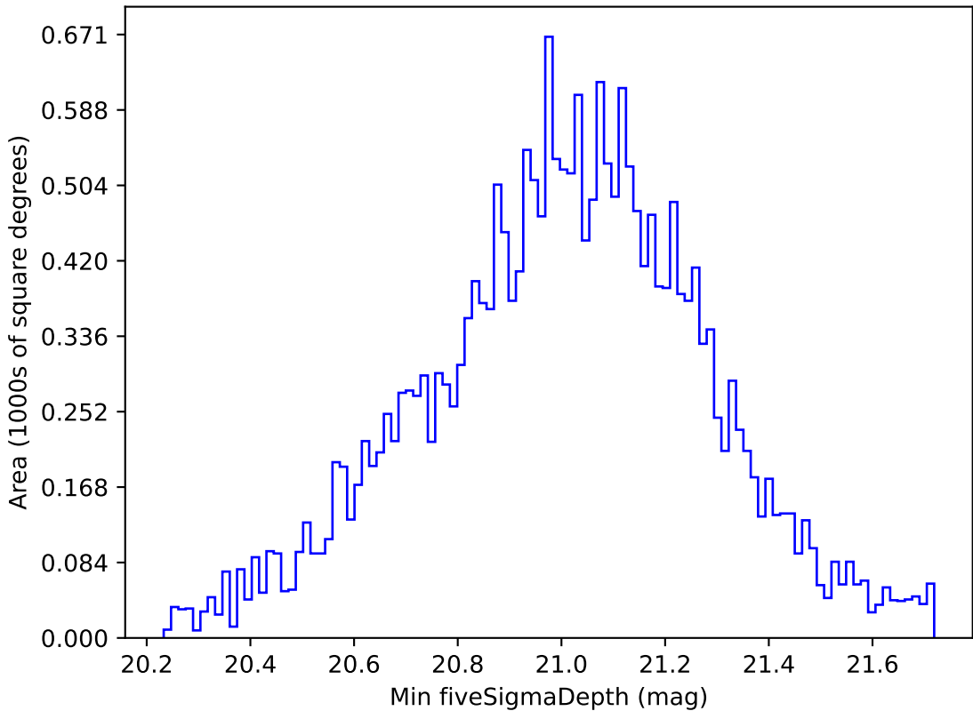
noroll_mjdp180_v3.4_10yrs All sky y band: Min fiveSigmaDepth
