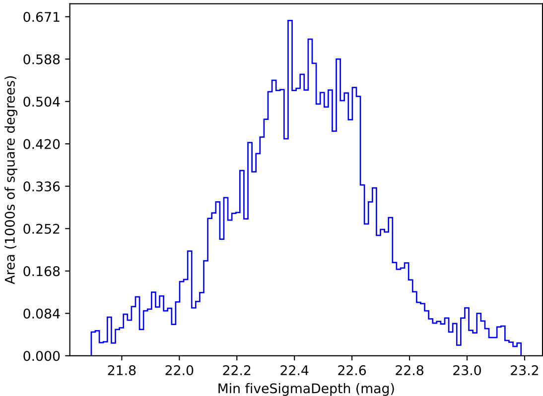
noroll_mjdp180_v3.4_10yrs All sky u band: Min fiveSigmaDepth
