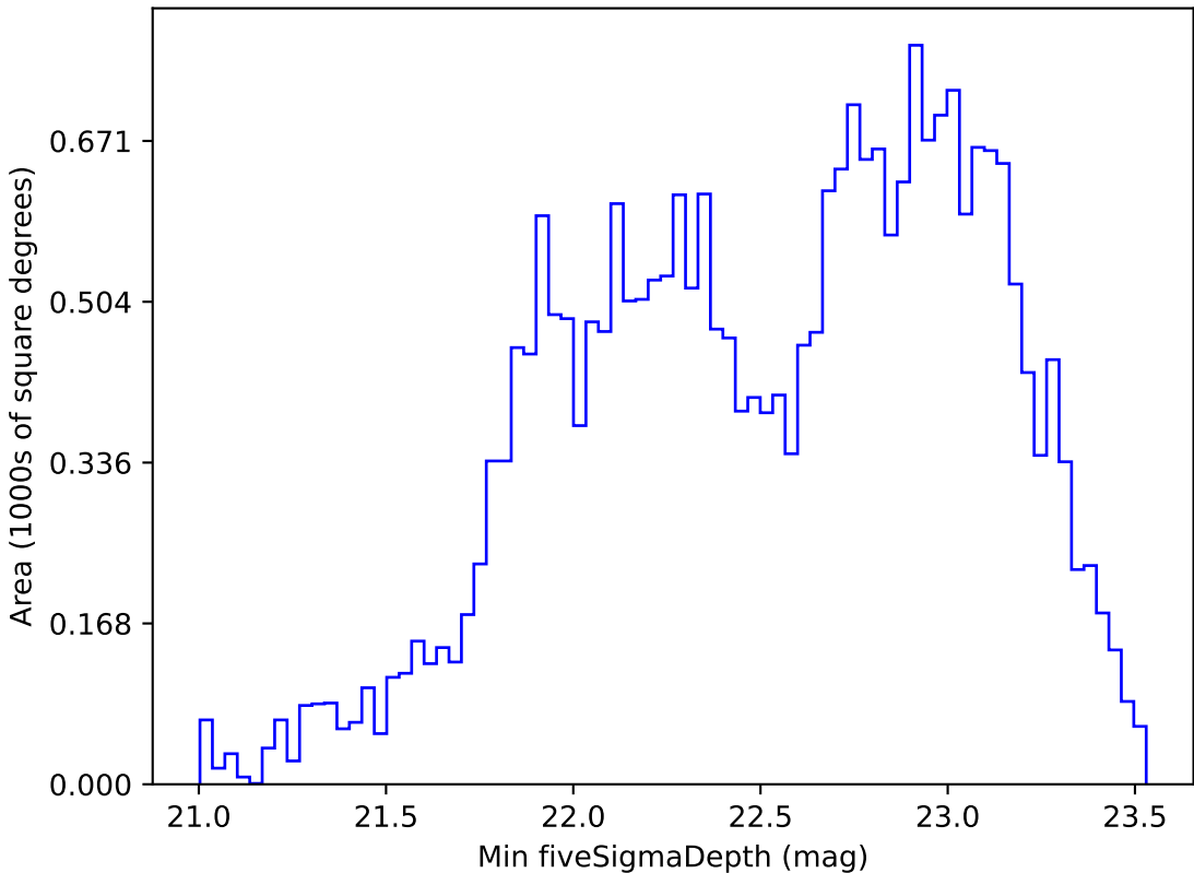
noroll_mjdp180_v3.4_10yrs All sky r band: Min fiveSigmaDepth
