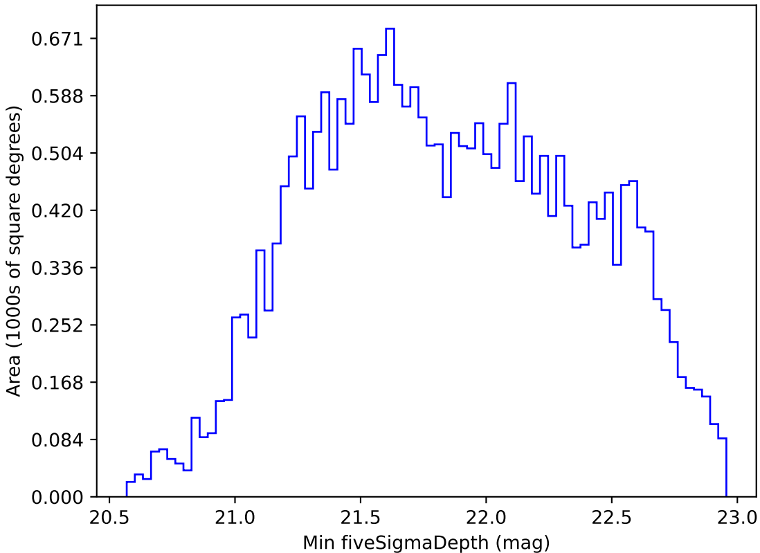
noroll_mjdp180_v3.4_10yrs All sky i band: Min fiveSigmaDepth
