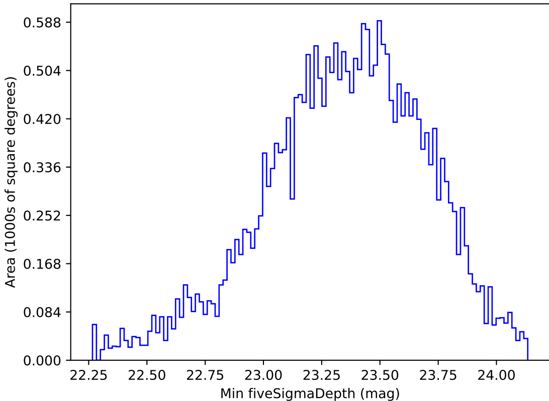
noroll_mjdp180_v3.4_10yrs All sky g band: Min fiveSigmaDepth
