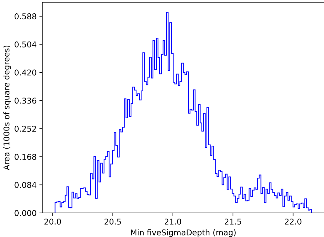
noroll_mjdp180_v3.4_10yrs All sky all bands: Min fiveSigmaDepth
