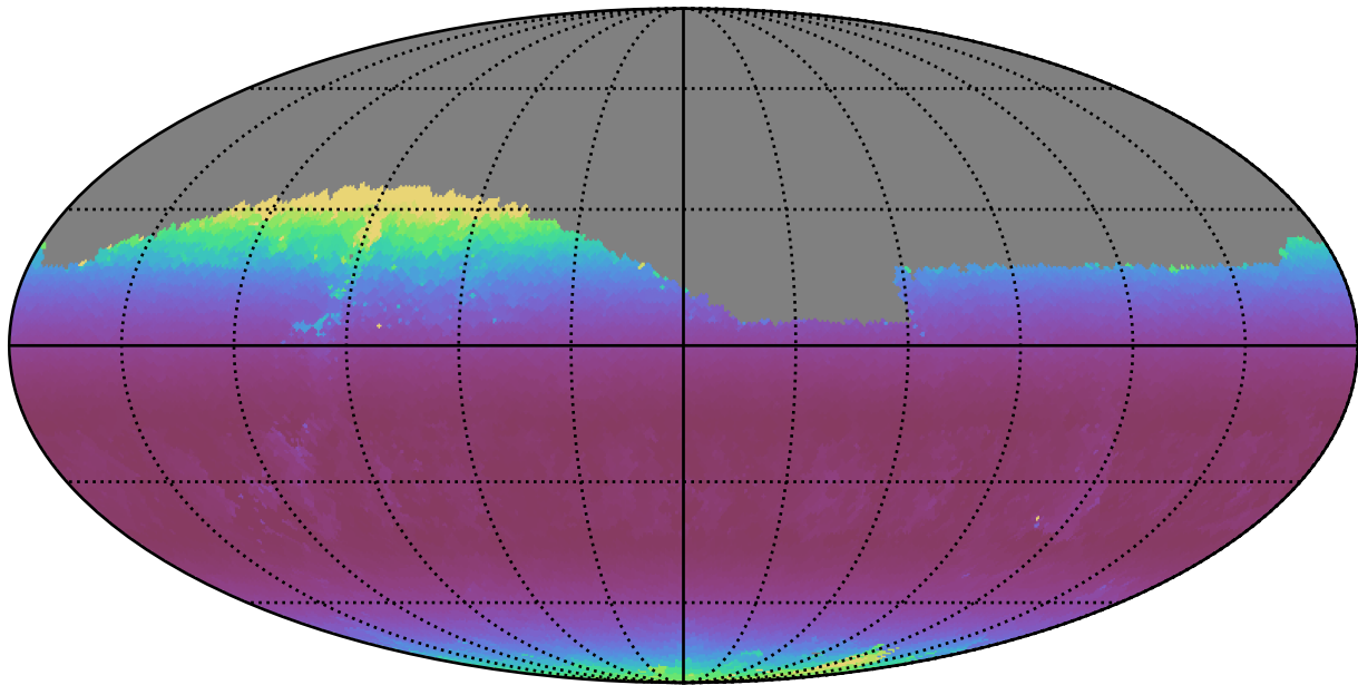
noroll_mjdp180_v3.4_10yrs Yr 1 z band: Min airmass
