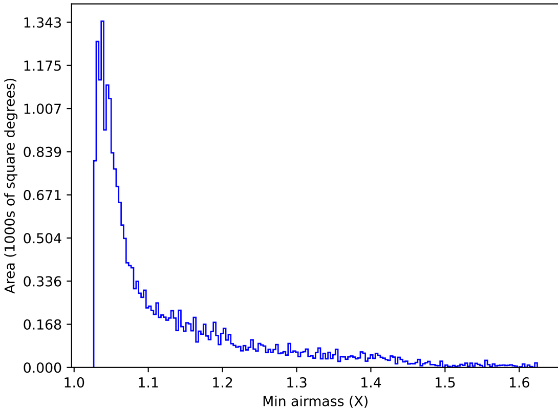
noroll_mjdp180_v3.4_10yrs Yr 1 y band: Min airmass
