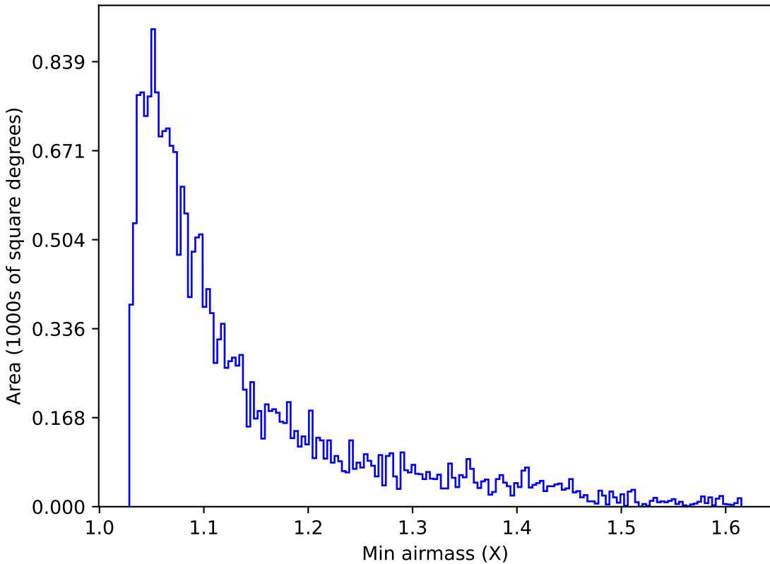
noroll_mjdp180_v3.4_10yrs Yr 1 u band: Min airmass
