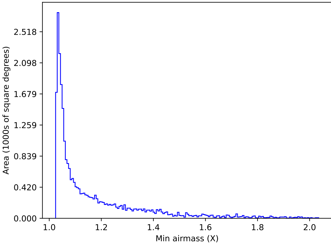
noroll_mjdp180_v3.4_10yrs Yr 1 r band: Min airmass
