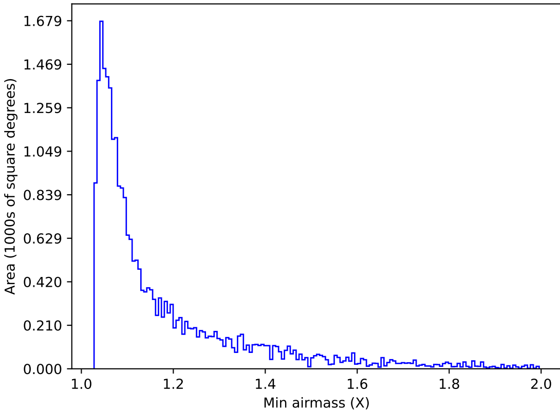
noroll_mjdp180_v3.4_10yrs Yr 1 g band: Min airmass
