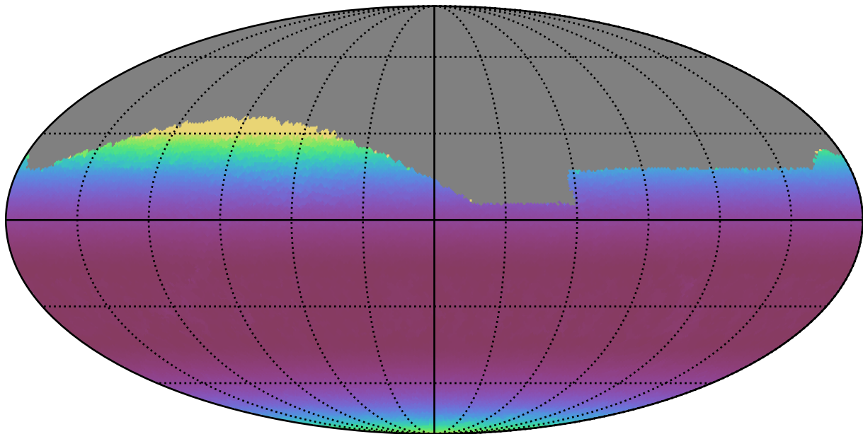
noroll_mjdp180_v3.4_10yrs Yr 1 all bands: Min airmass
