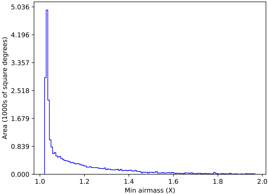
noroll_mjdp180_v3.4_10yrs Yr 1 all bands: Min airmass
