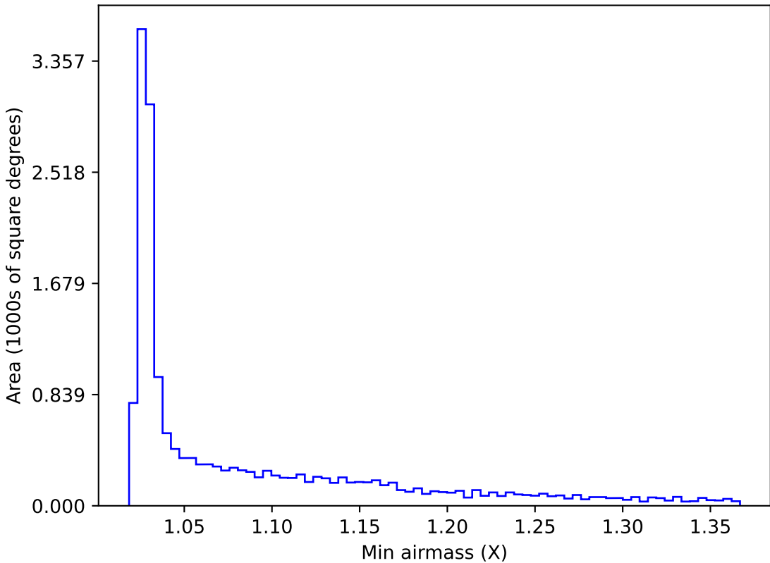
noroll_mjdp180_v3.4_10yrs WFD z band: Min airmass
