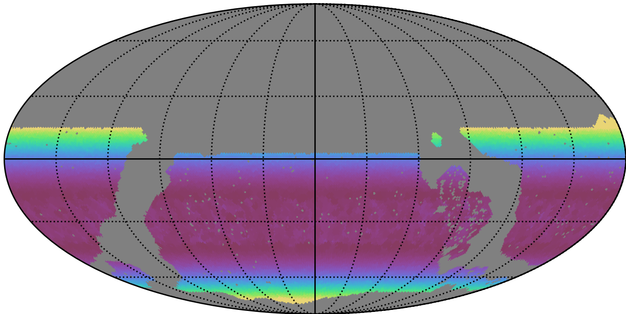
noroll_mjdp180_v3.4_10yrs WFD u band: Min airmass
