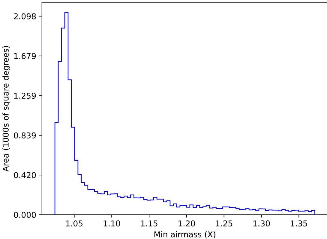
noroll_mjdp180_v3.4_10yrs WFD u band: Min airmass
