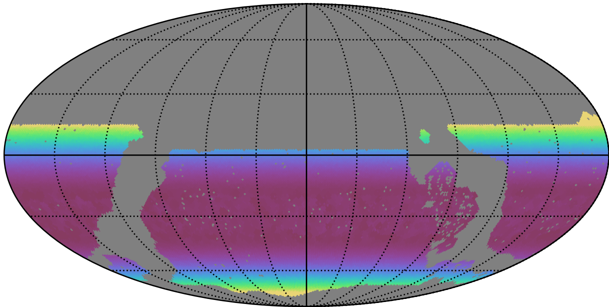
noroll_mjdp180_v3.4_10yrs WFD r band: Min airmass
