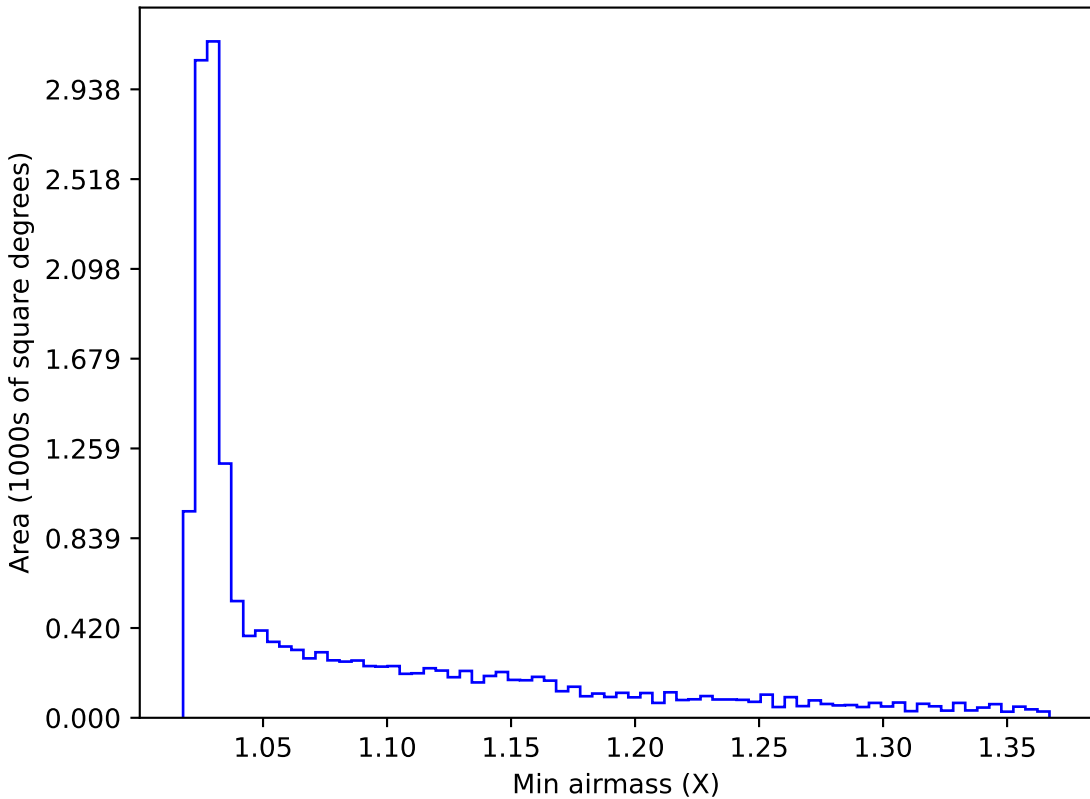
noroll_mjdp180_v3.4_10yrs WFD i band: Min airmass
