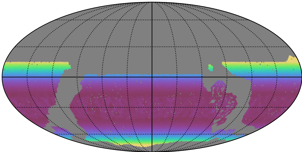
noroll_mjdp180_v3.4_10yrs WFD g band: Min airmass
